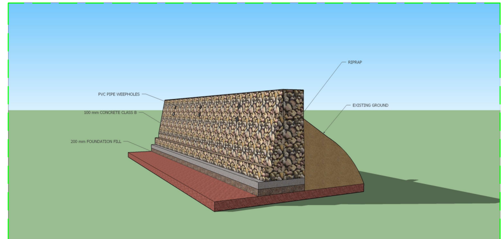
CONSTRUCTION OF RIPRAP ATLEAST 280 l.m. LENGTH
